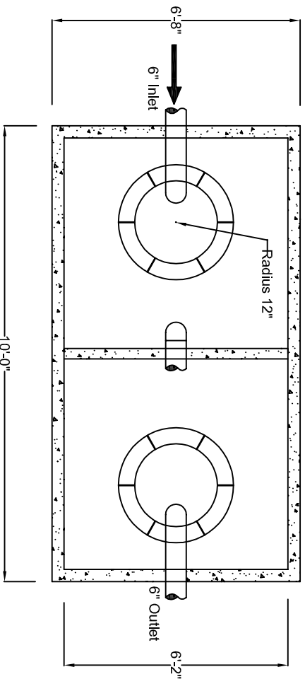
PLAN VIEW
